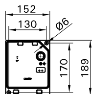
MARVIK 3,6 MOUNTING DETAIL
